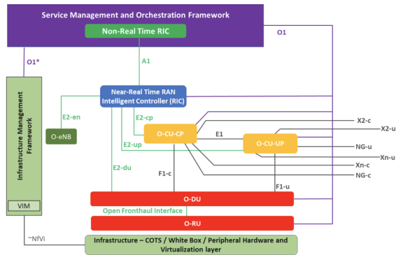
Figure 2: O-RAN architecture overview
