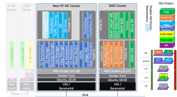
Figure 1: Demo deployment architecture
